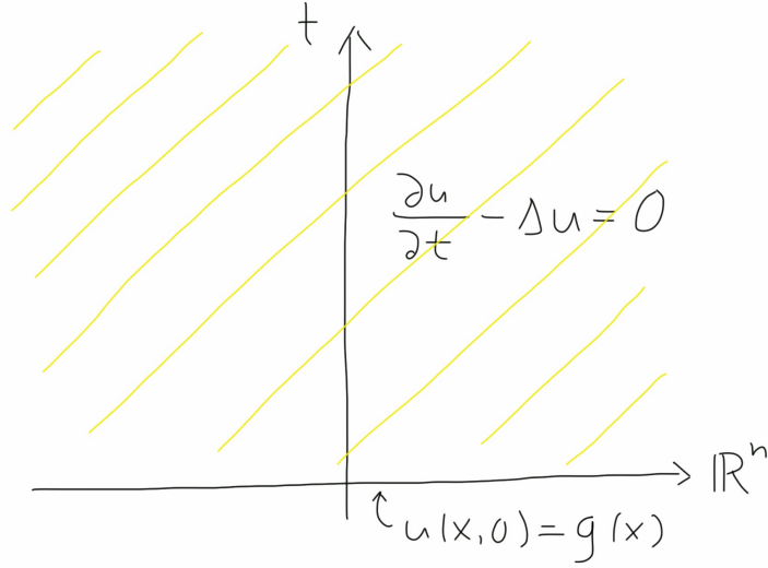
Figure 3.5: The heat equation in the upper half-space.
