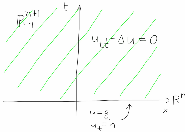
Figure 6.3: The Cauchy problem for the wave equation.
