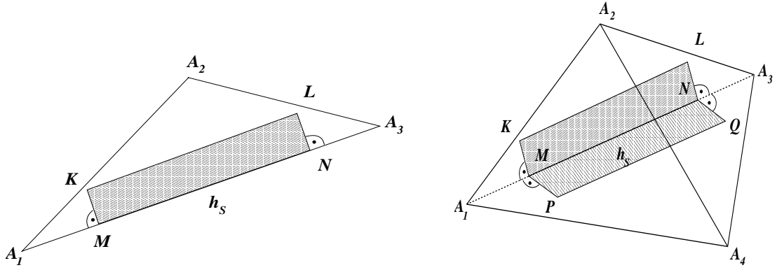
Figure 1: Illustration for the proof (4) \implies (1).
