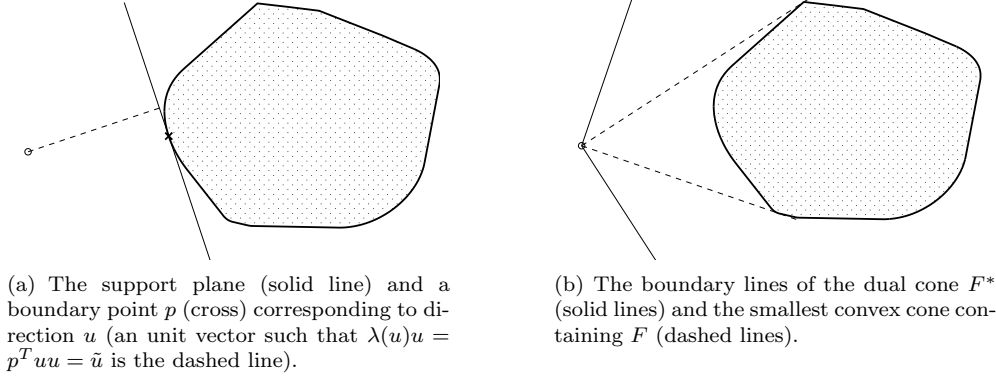
FIG. 3.1. A k = 2 dimensional F (thick outline). The origin is marked with a circle.
